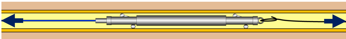
Figure 23: Inclinometer sent to the far end within casing with tension applied to both the pull rope and the cable to stop either of them going slack
