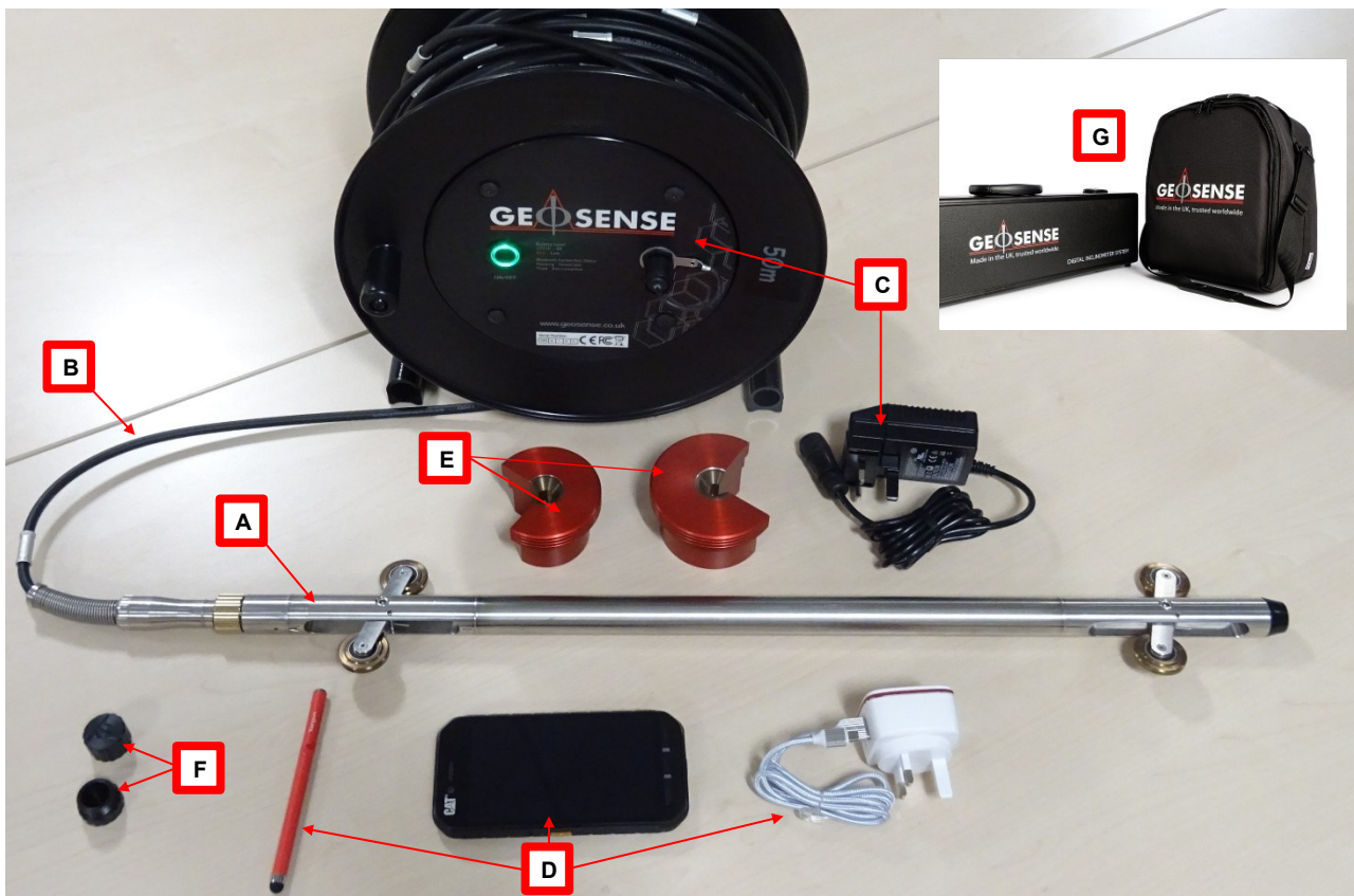
Figure 5: Inclinometer Components
