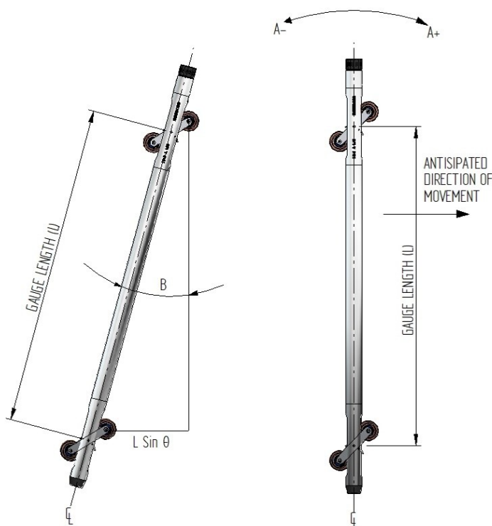
Figure 3: L \sin \theta and Roll Planes of Measurement
